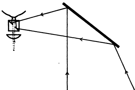
Fig. 57. Optical construction of Abbe camera lucida.
